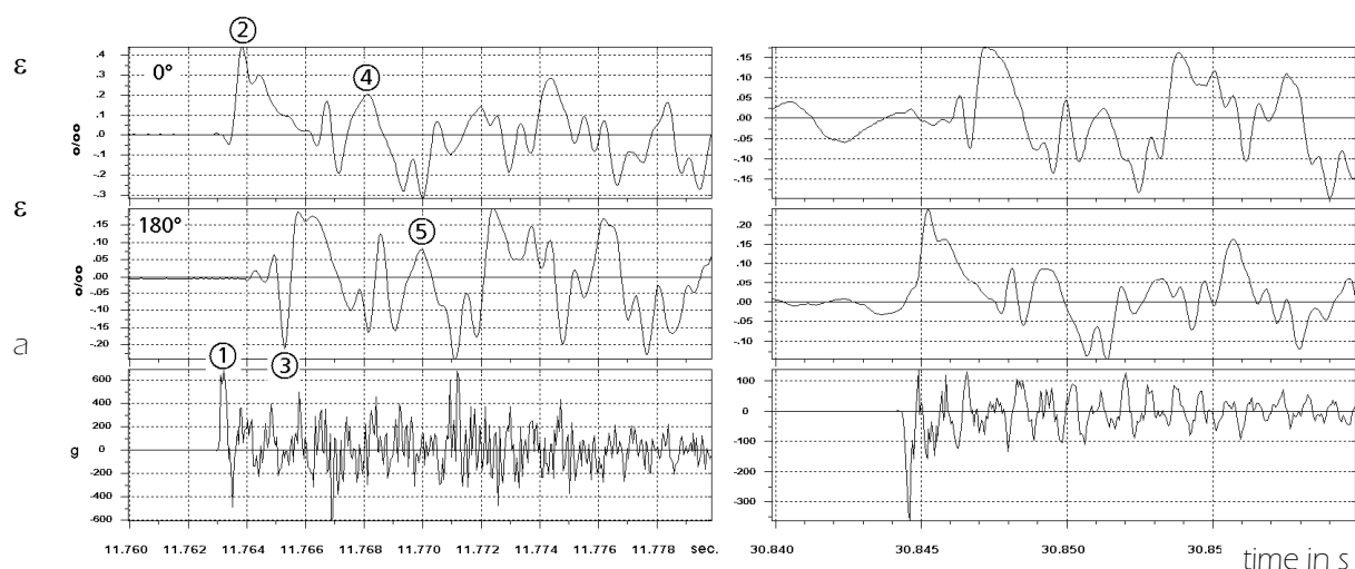
Fig. 5. Time histories of strains on bell and clapper acceleration
