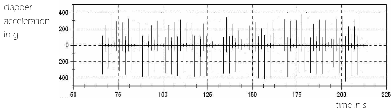
Fig 6: Acceleration during 150s ringing
