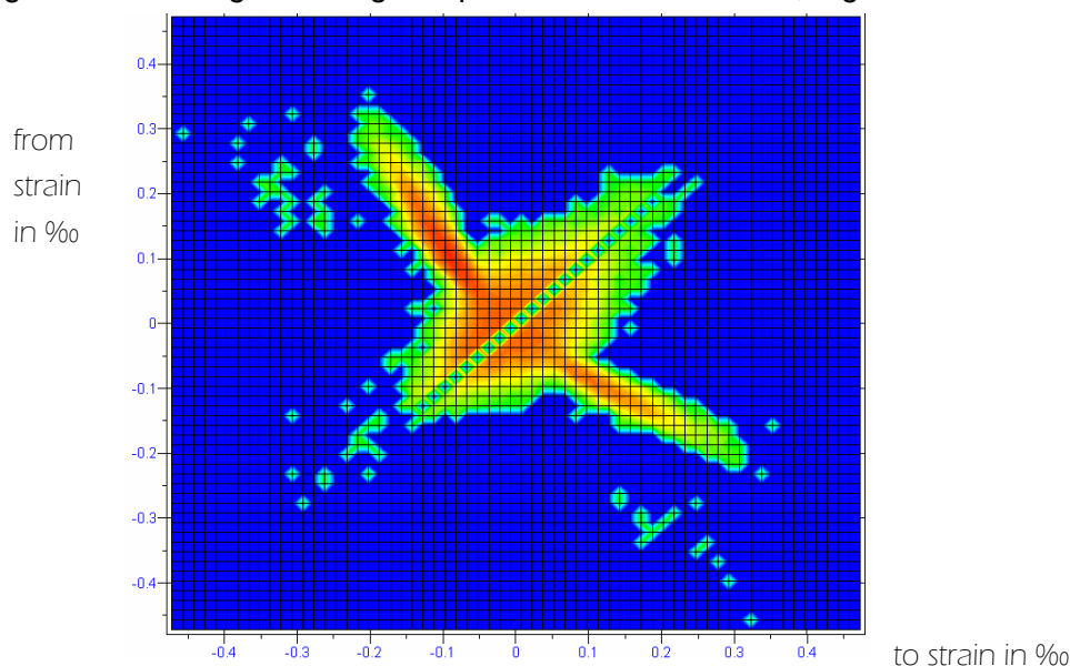
Fig. 7: Rainflow matrix of strain outside sound burp opposite to clapper impact, 1min
