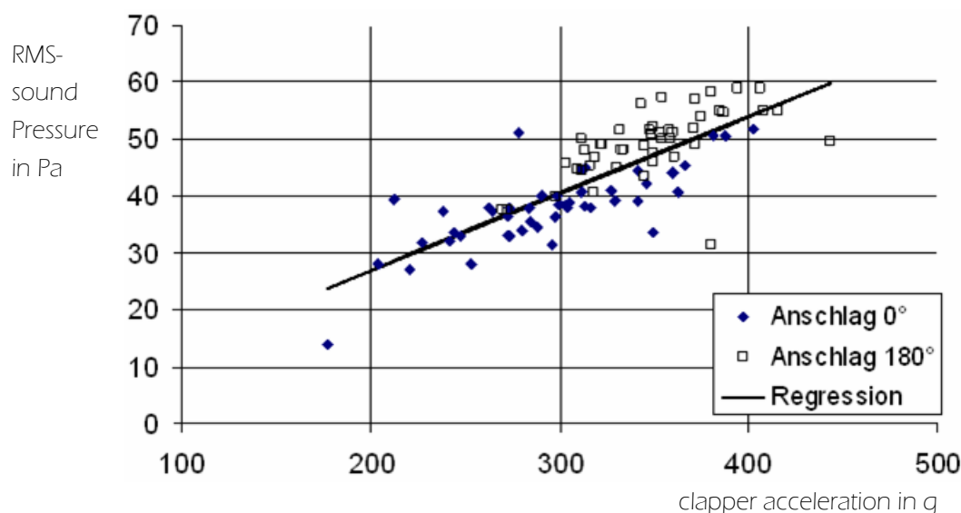
Fig. 10: Correlation of sound pressure and clapper acceleration
