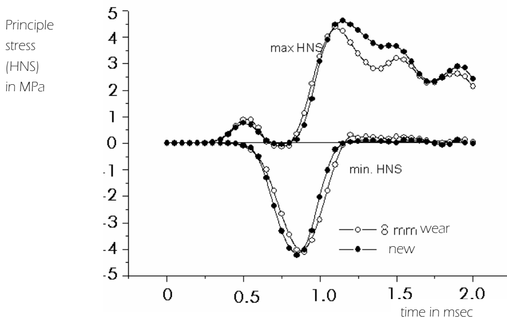
Fig. 13: Principle stresses at the sound burp during clapper impact on a new and bell with wear
