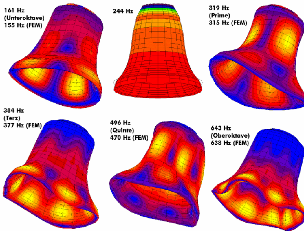
Fig. 12: Modal analysis of a bell for verification of the model [1]
