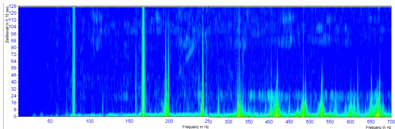
Fig. 11: Waterfall diagram, power spectral density of the sound pressure over about 20 sec after clapper stroke
